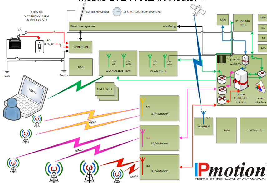
CAR-A-WAN.coach v6 /CAR-A-WAN.112 v6 Blockschaltbild block diagram / diagramme de bloc Mobile LTE-A WLAN Router GPS
