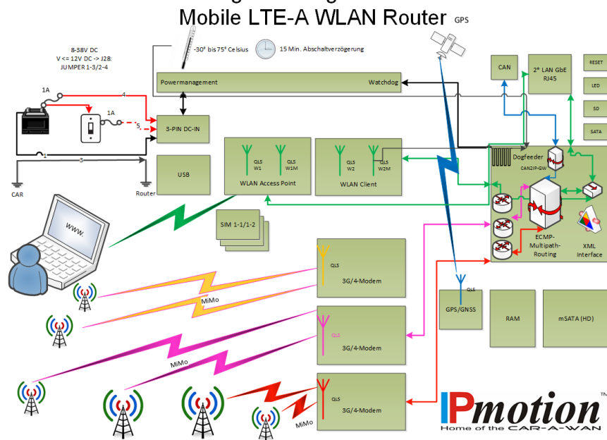
CAR-A-WAN.coach v6 /CAR-A-WAN.112 v6 Blockschaltbild block diagram / diagramme de bloc
